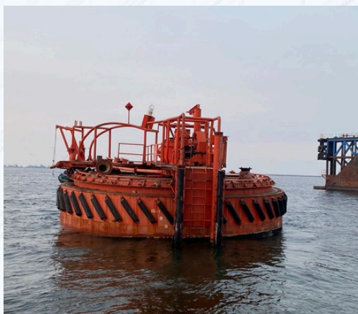
FLOATING REPAIR OF SINGEL POINT MOORING Location : Cilincing, Jakarta Utara
